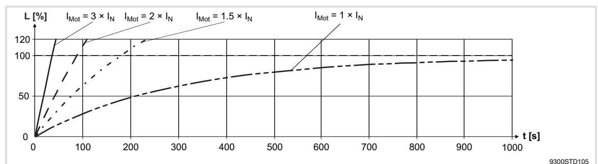
Fig. 2-28 I^2 \times t -monitoring: Release times for different motor currents and trigger thresholds
