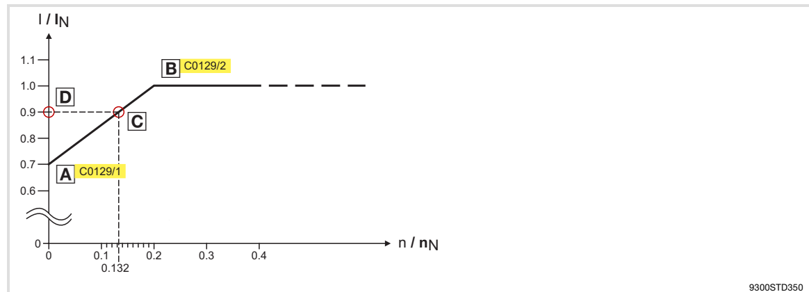
Fig. 2-29 Working point in the range of characteristic lowering
