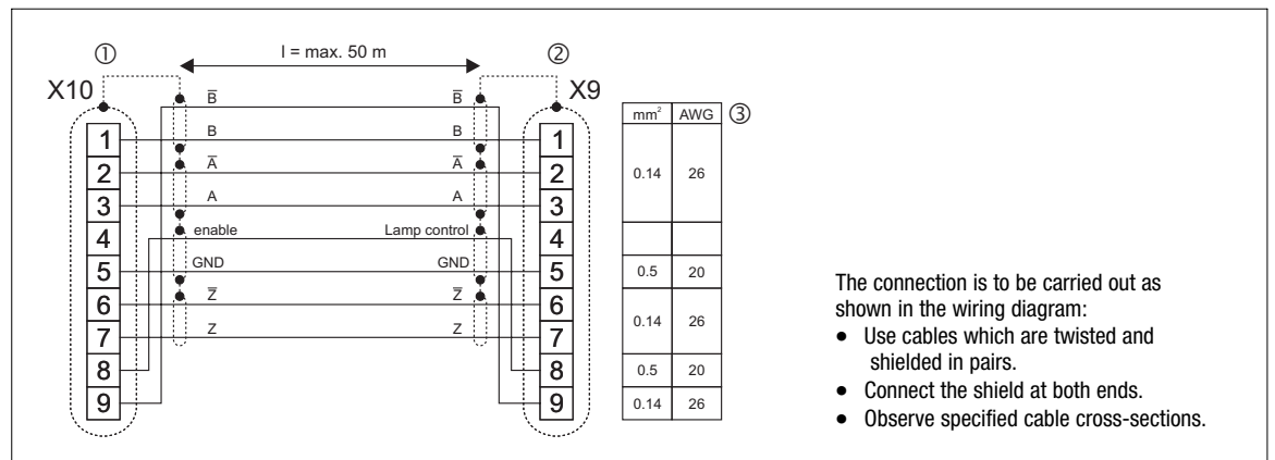
Connection of digital frequency output X10 with digital frequency input X9
