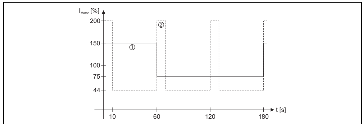
Overcurrent diagram
