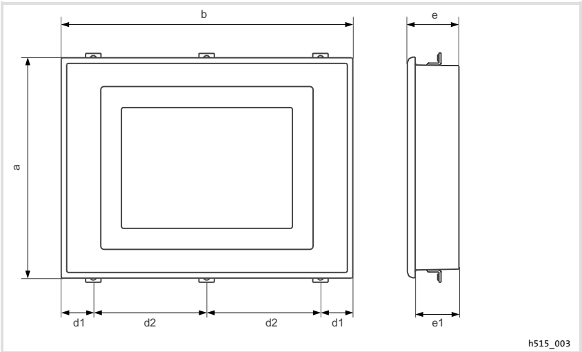
Fig.2-2 Dimensions
