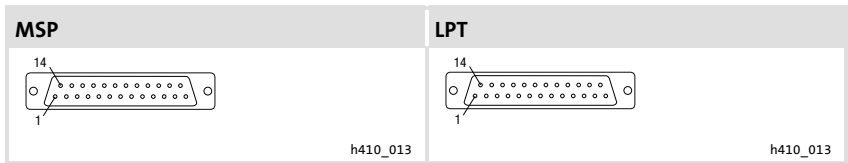
Fig.2-1 DB25 socket
