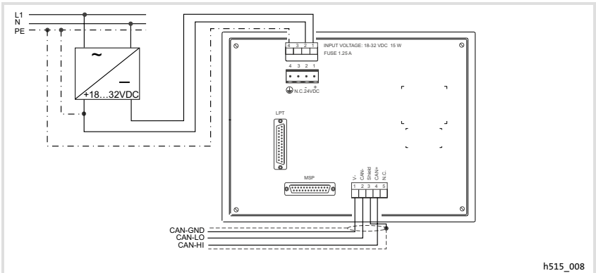
Fig.4-1 Assignment of the terminals
