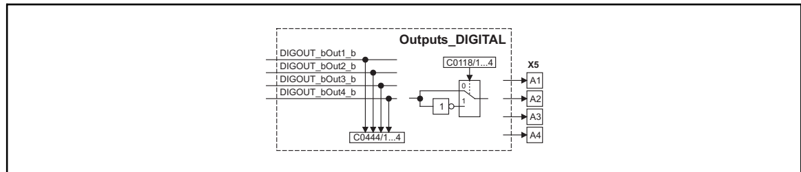
Fig. 2-22 Outputs_DIGITAL
